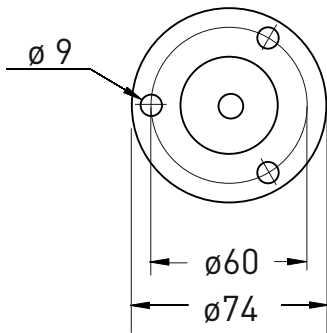
DETAIL MARINE FEET Section A-A
