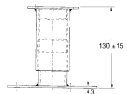
DETAIL MARINE FEET
